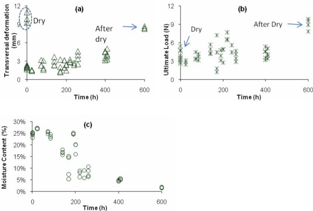
Figure 5: Transversal deformation test results. (a) transversal deformation x time, (b) ultimate load x time and (c) moisture content x time
