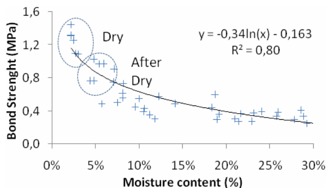
Figure 7: Bond Strength x Moisture Content
