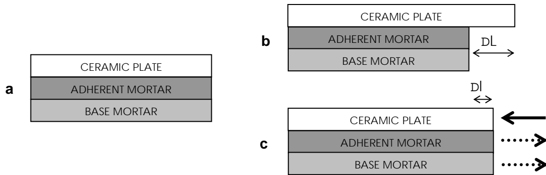
Figure 2 – diagram of acting stresses on the system due to the action of water on the ceramic linings (a – dry condition; b – plate water saturation (free layers – hypothetical); c – real behavior owing to solidarity between layers).
