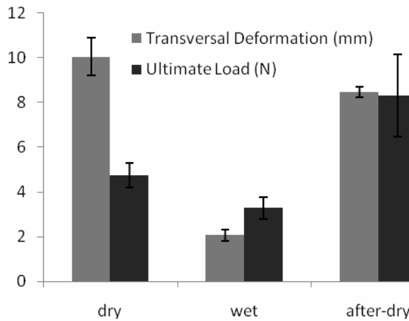
Figure 4: Average results in the transversal deformation test.
