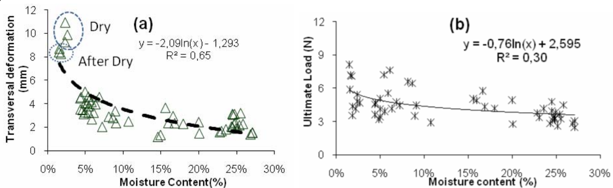
Figure 6: Results for the transversal deformation test. (a) Flexibility and (b) Ultimate load
