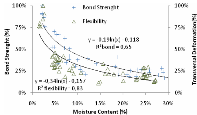
Figure 8: Normalized results for the bond strength and transversal deformation
