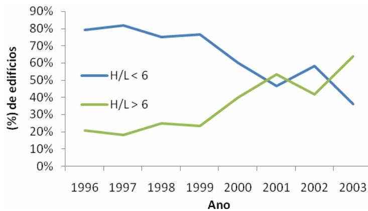
Figure 1: Variation of the slenderness rates in buildings (H /L) in the city of Recife along the years [5] . H= building height and L= building width.
