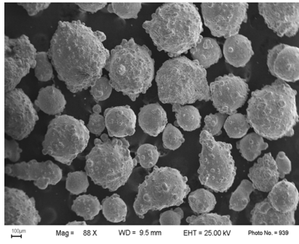
Figure 1. SEM micrograph of the stainless-steel particles.
