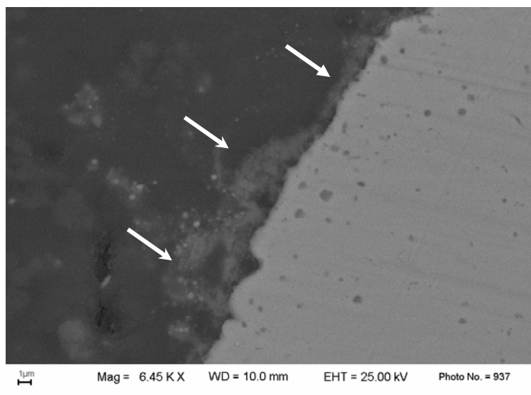
Figure 8. SEM micrographs of the polished surface of Mix2, the chromium rich layer is arrowed.
