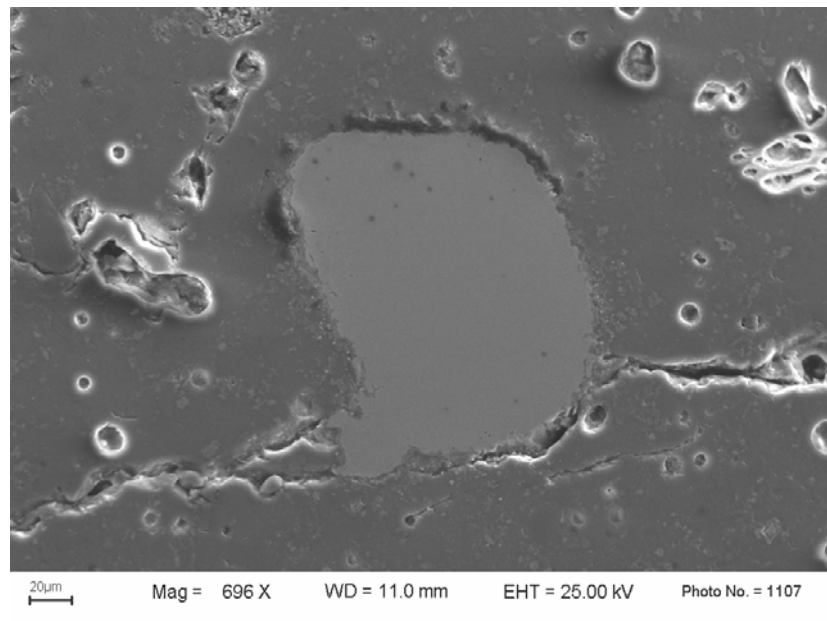
Figure 6. SEM micrographs of the polished surface of Mix3, showing a crack deflected around metal particles.
