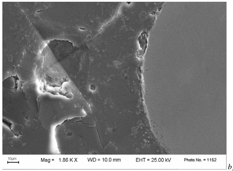
Figure 7. SEM micrographs of the polished surface of Mix3: a) crack deflection, b) magnification.
