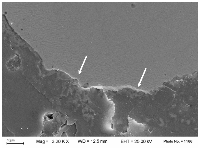
Figure 5. SEM micrographs of the polished surface of Mix3, crack path blunt by a metal particle. The arrows underline the metal detachments.
