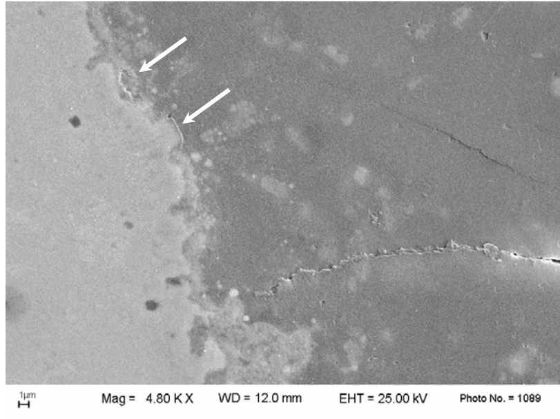
Figure 4. SEM micrographs of the polished surface of Mix2, crack path blunt by a metal particle. The arrows underline the metal detachments.
