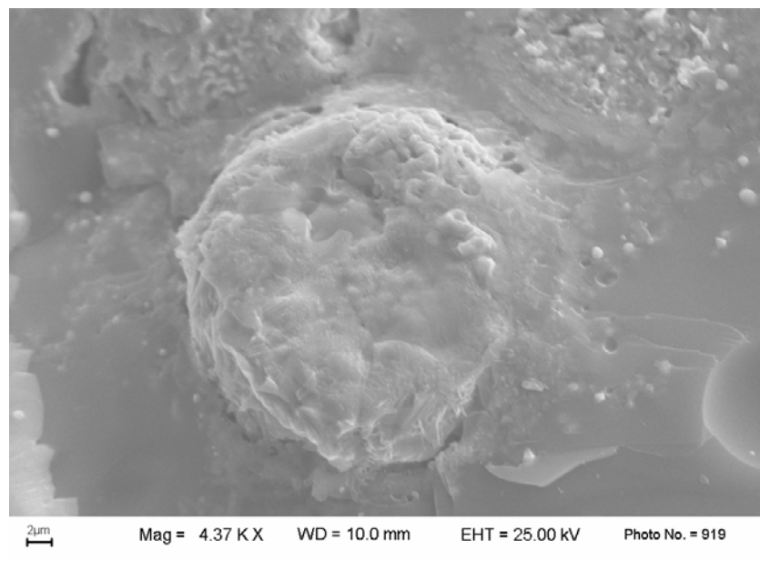
Figure 2. SEM micrograph of Mix2, a round metal particle good adhering to the ceramic matrix.
