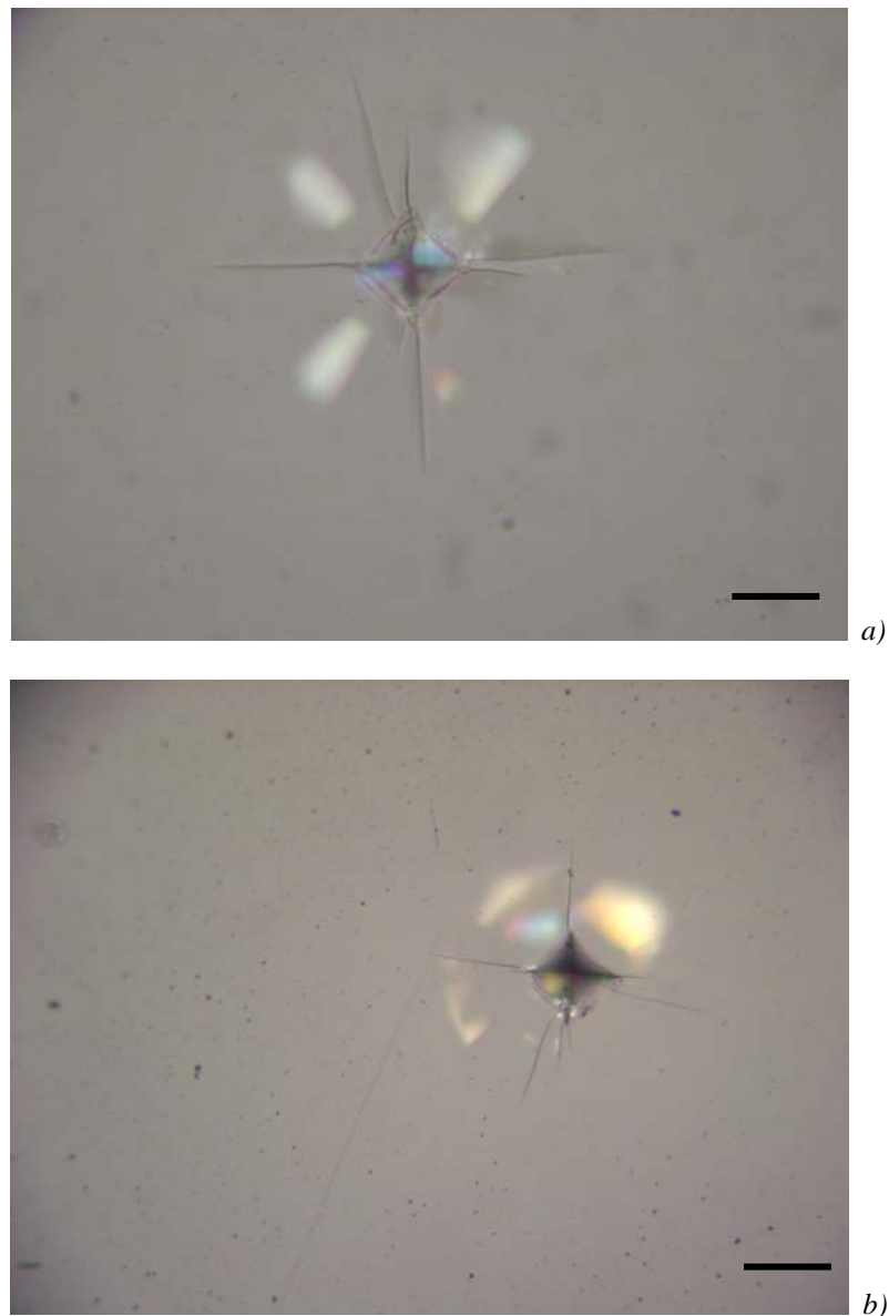
Figure 5. Light micrographs of Vickers indentations and the corresponding crack path of a) S-L G and, b) Red samples in air environment. The bar is 50 \mu\text{m} .
