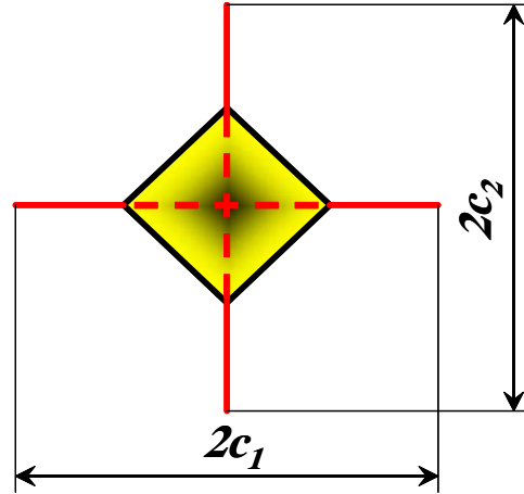
Figure 3. Vickers impression and median-radial cracks.
