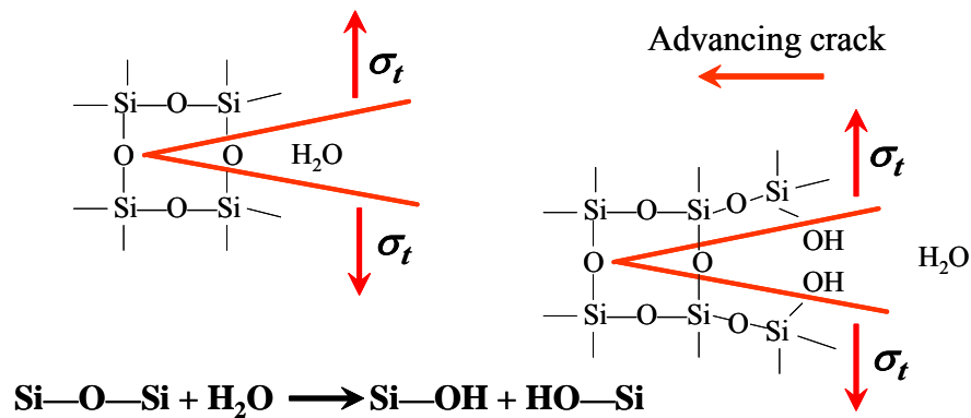
Figure 1. Qualitative molecular model of crack propagation in soda-lime glass.
