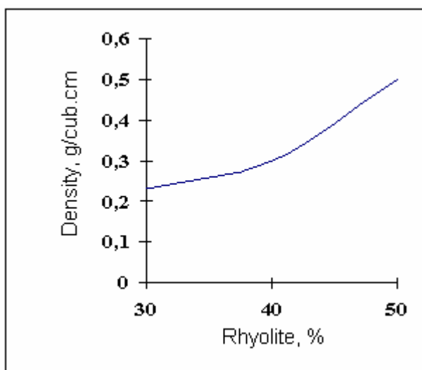
Fig. 1. Dependence of density of the material on the contents of rhyolite
