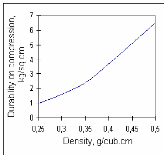
Fig. 2. Dependence of durability on compression from porosity of the material
