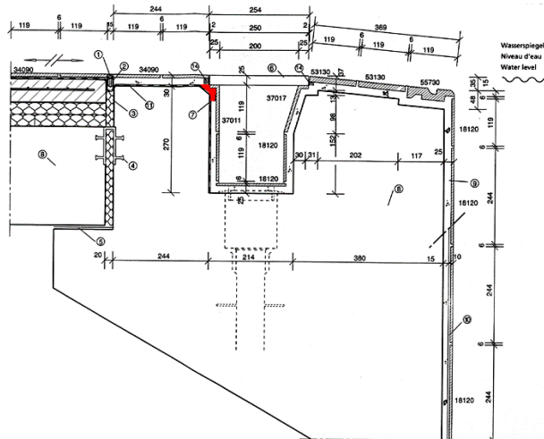
Image 6: A capillary break of epoxy resin (marked in red) at the pool head prevents water penetrating from the pool ...
